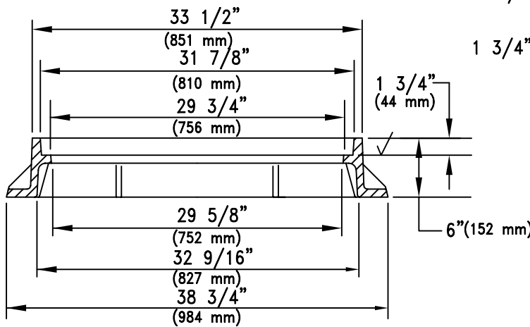
FRAME SECTION A-A
