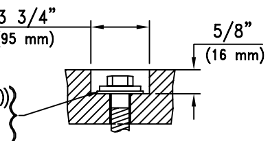
PICKBAR RECESS DETAIL
