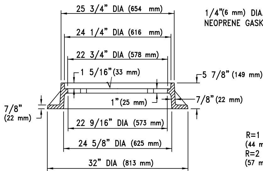
FRAME SECTION A-A √ DENOTES MACHINED SURFACE
