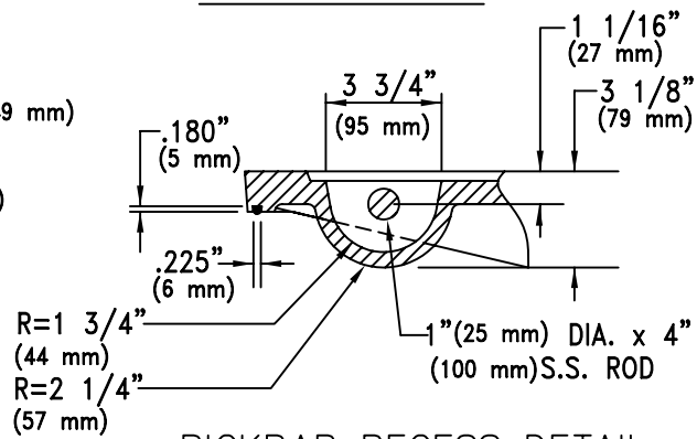
PICKBAR RECESS DETAIL
