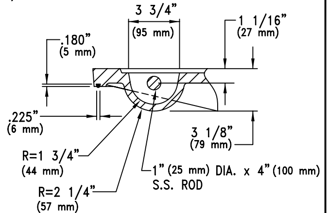
PICKBAR RECESS DETAIL
