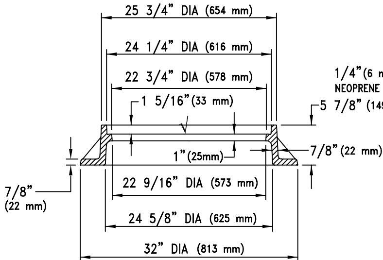
FRAME SECTION A-A
